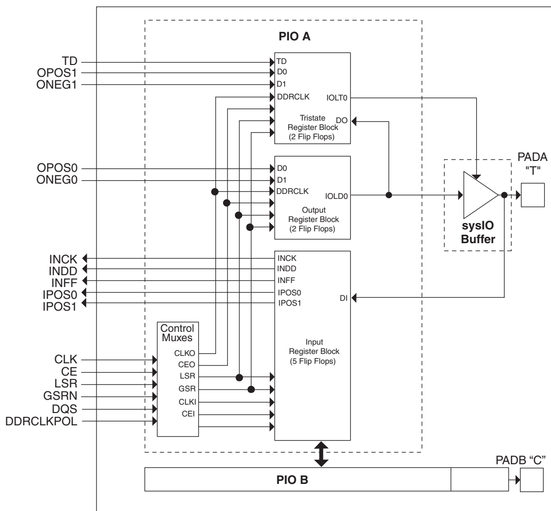
Figure 2-17. PIC Diagram
