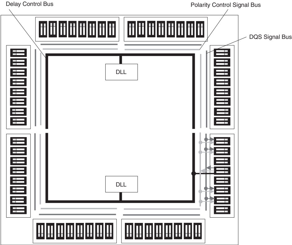
Figure 2-27. DLL Calibration Bus and DQS/DQS Transition Distribution
