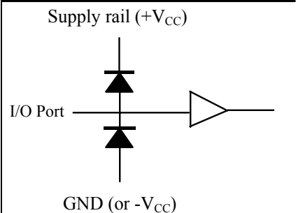
Steering Diode Application FIGURE 1
