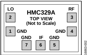
Figure 2. Pin Configuration
