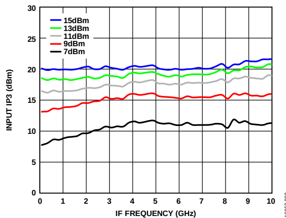
Figure 76. Input IP3 vs. IF Frequency at Various LO Power Levels, T_A = 25^\circ\text{C}
