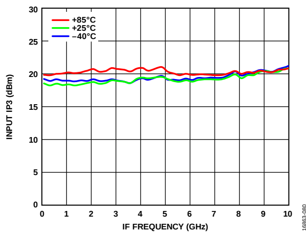
Figure 74. Input IP3 vs. IF Frequency at Various Temperatures, LO = 13 dBm
