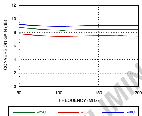
Figure 45. Conversion Gain vs. IF Frequency @ RF=1900 MHz, VGATE=5V [1]
