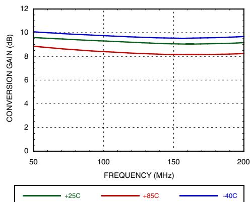
Figure 43. Conversion Gain vs. IF Frequency @ RF=900 MHz, VGATE=5V [1]
