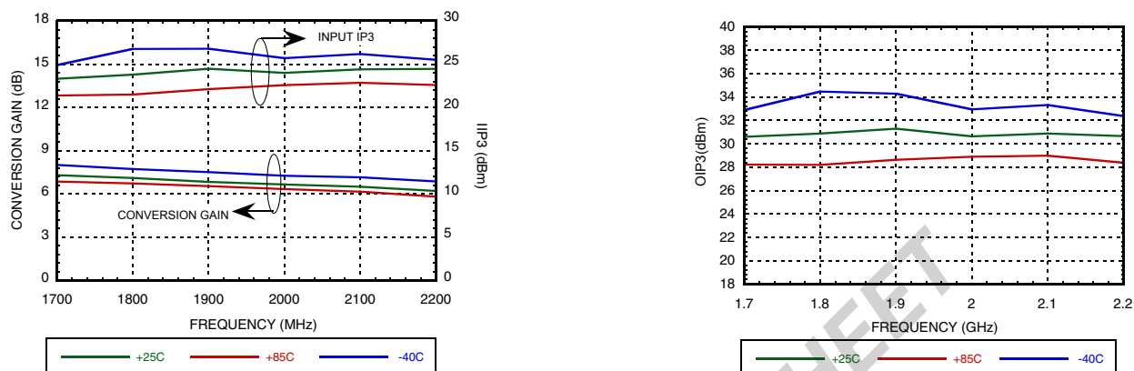
Figure 78. Conversion Gain, IIP3 and OIP3 for 1900MHz RF frequency band. [1]
