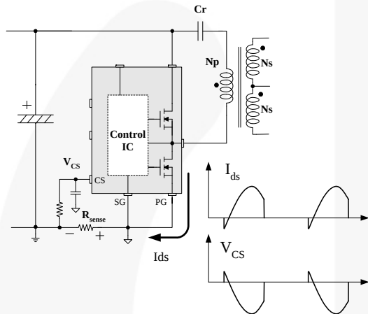
Figure 23. Half-Wave Sensing
