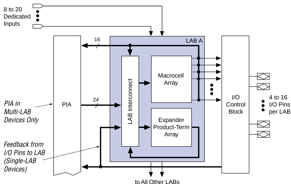
Figure 1. MAX 5000 Architecture
