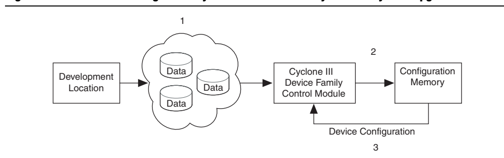
Figure 9-32. Functional Diagram of Cyclone III Device Family Remote System Upgrade
