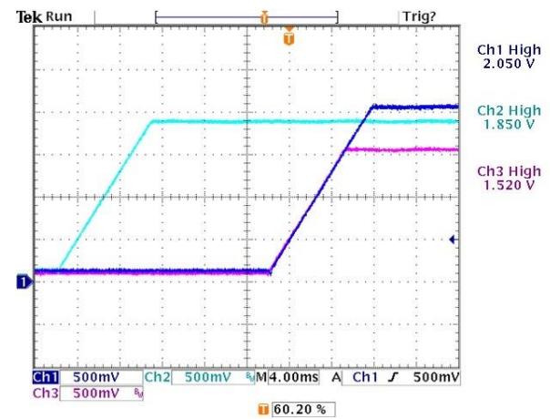
Figure 17. Turn-On with Different Rising Slew Rates. Rising Slew Rates are V1-1V/ms, V2-0.5V/ms, V3-0.2V/ms.
