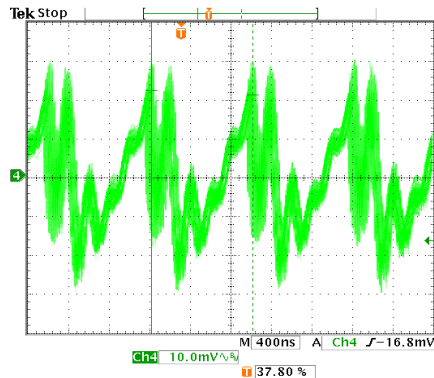
Figure 38. Input Voltage Noise, No Interleave
