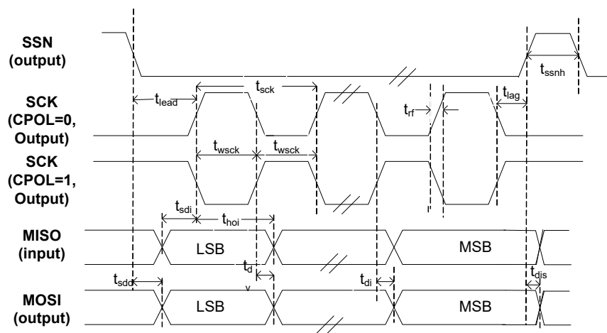
Figure 5. SPI Timing
