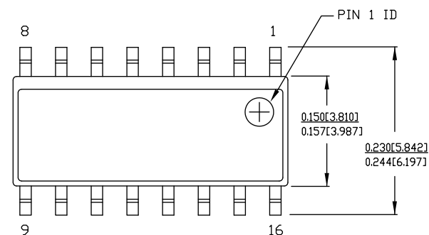
Figure 8. 16-pin SOIC (150 Mils) Package Outline
