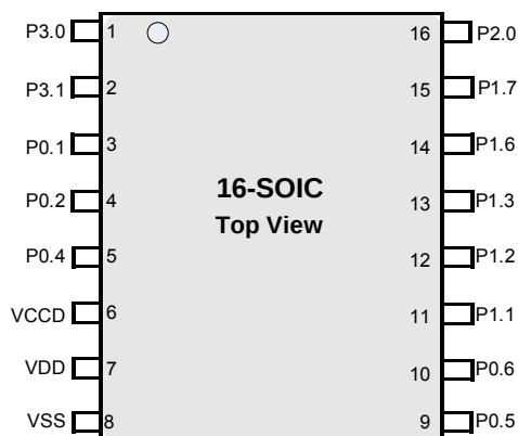
Figure 4. 16-pin SOIC Pinout
