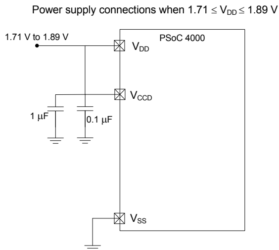
Figure 6. 24-pin QFN Bypass Scheme Example - Regulated External Supply
