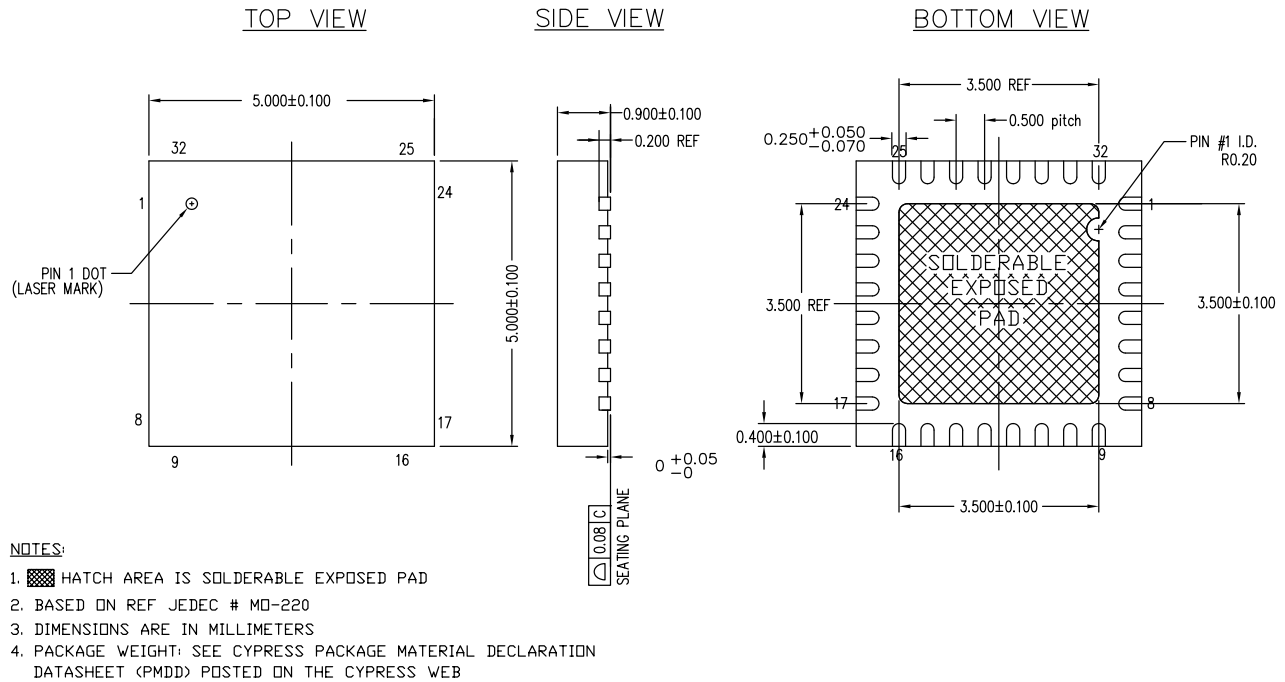
Figure 16. 32-pin QFN ((5 × 5 × 1.0 mm) 3.5 × 3.5 E-Pad (Sawn)) Package Outline, 001-30999
