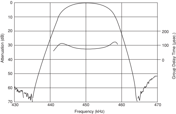
IFT+CFULA450KF1Y-B0
