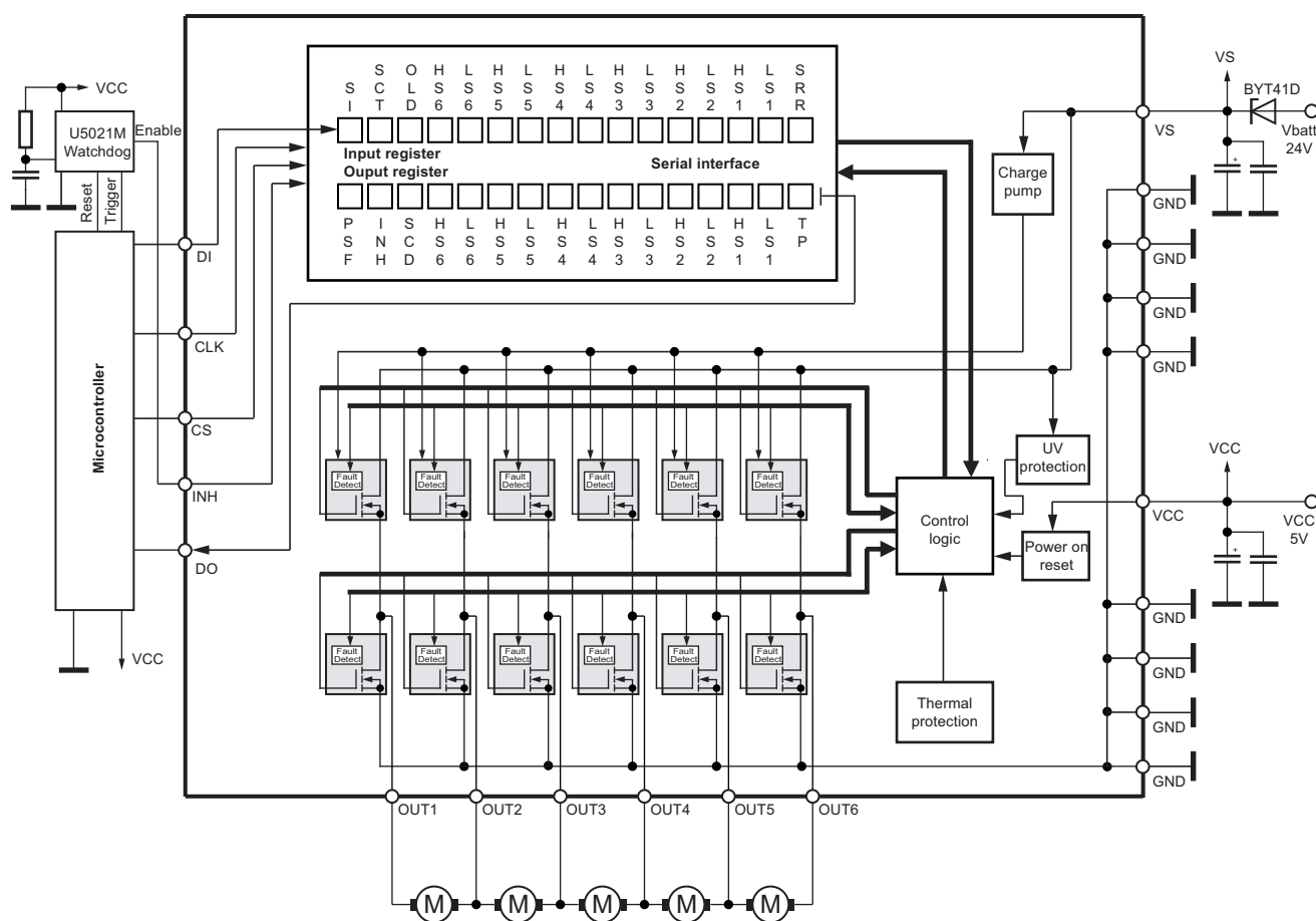
Figure 10-1. Application Circuit
