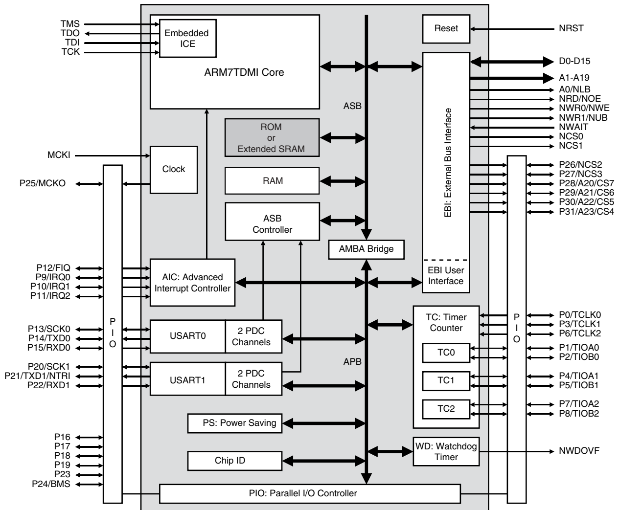
Figure 2. AT91X40 Series
