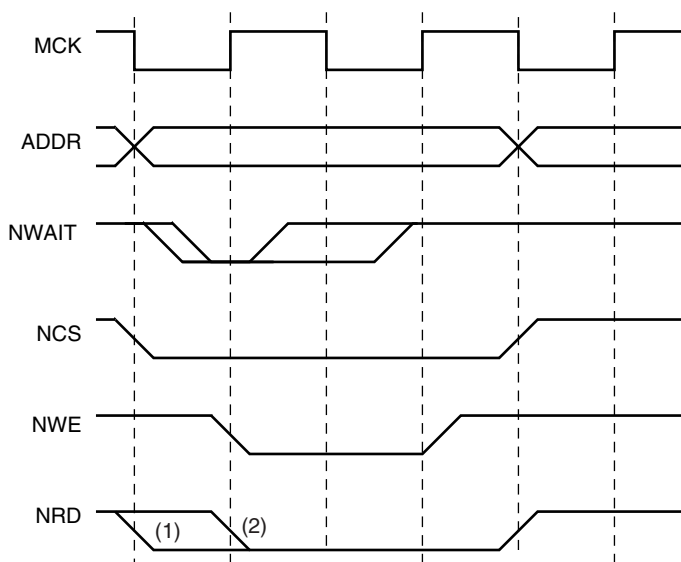
Figure 20. External Wait
