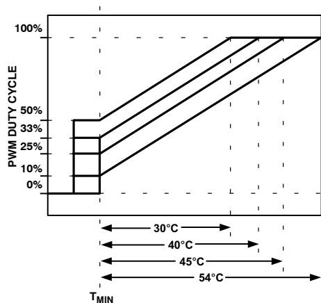
Figure 59. Increasing PWM MIN Changes Effective T_{\text{RANGE}}
