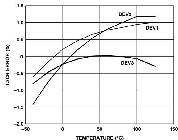
Figure 18. TACH Accuracy vs. Temperature
