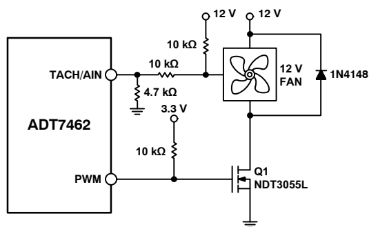
Figure 40. Driving a 3-Wire Fan
