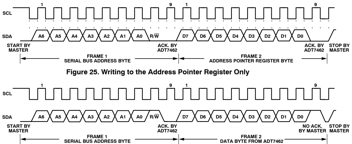
Figure 26. Reading Data from a Previously Selected Register
