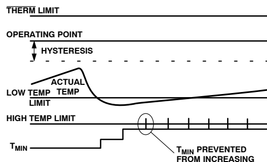
Figure 73. T_{MIN} Adjustments Limited by High Temperature Limit
