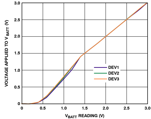
Figure 16. Applied Voltage vs. V BATT Reading
