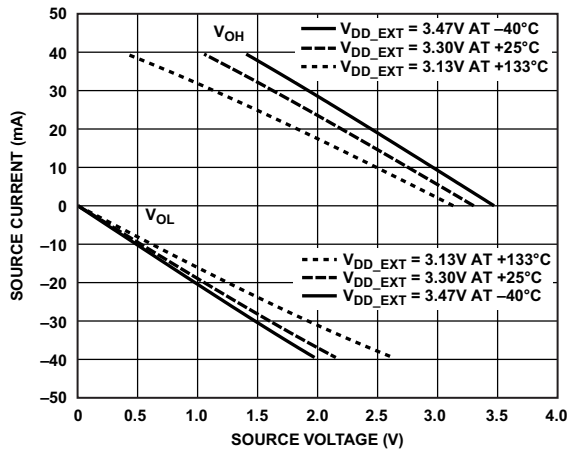
Figure 82. Driver Type A Current ( 3.3\text{ V } V_{DD\_EXT} )
