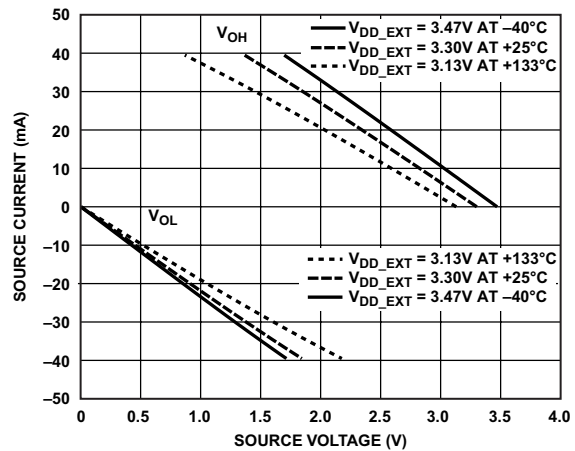
Figure 84. Driver Type H Current ( 3.3\text{ V } V_{DD\_EXT} )
