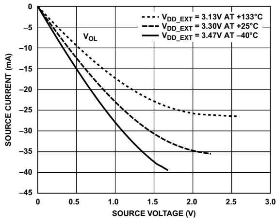
Figure 83. Driver Type D Current ( 3.3\text{ V } V_{DD\_EXT} )
