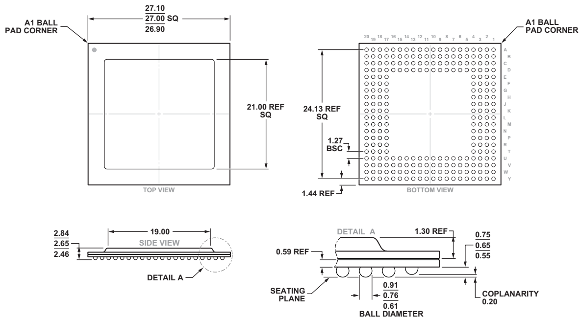
Figure 51. 256-Ball Ball Grid Array, Thermally Enhanced [BGA_ED] (BP-256-2) Dimension shown in millimeters
