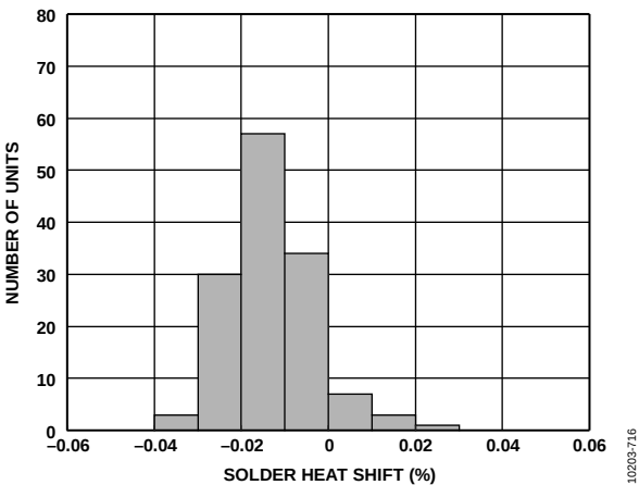
Figure 17. ADR4520 Solder Heat Resistance Shift (3 x Reflow)
