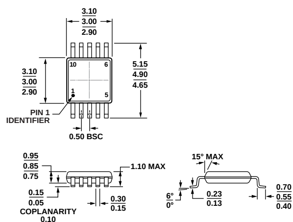
COMPLIANT TO JEDEC STANDARDS MO-187-BA Figure 30. 10-Lead Mini Small Outline Package [MSOP] (RM-10) Dimensions shown in millimeters
