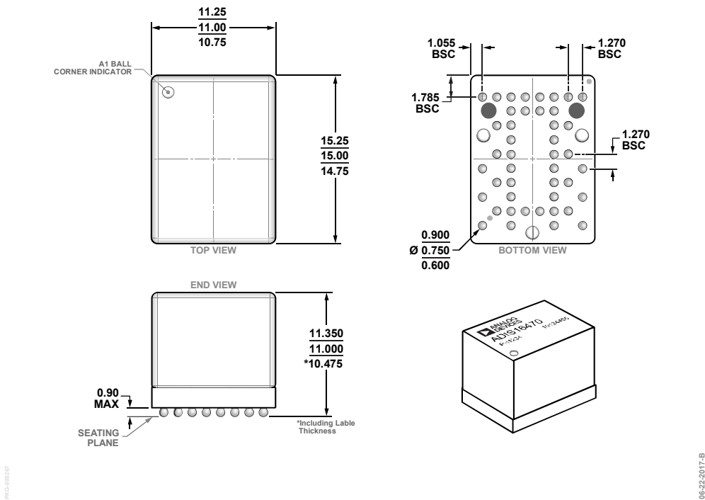
Figure 51. 44-Ball Ball Grid Array Module [BGA] (ML-44-1) Dimensions shown in millimeters
