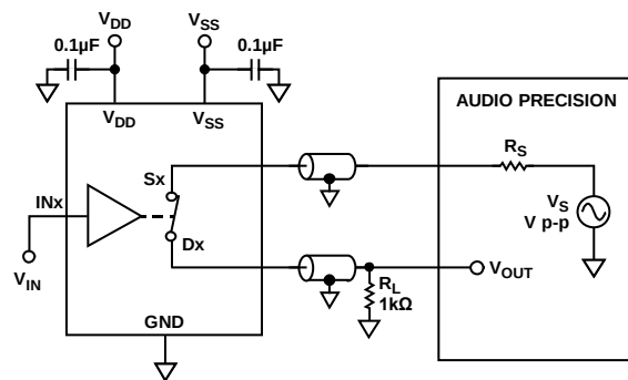
Figure 27. THD + Noise
