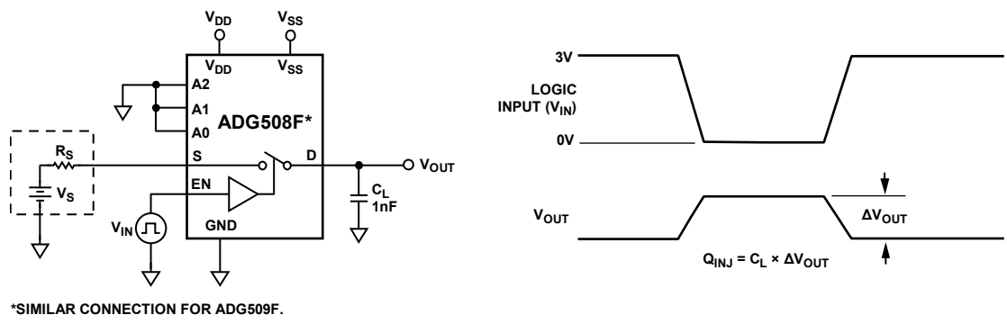
Figure 30. Charge Injection
