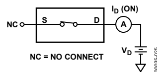
Figure 24. I_D (On)
