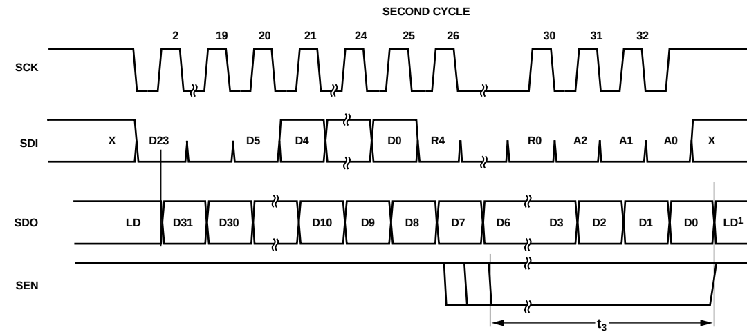
Figure 32. Open Mode: Serial Port Timing Diagram, Read Operation, Second Cycle
