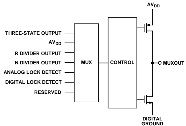
Figure 32. MUXOUT Schematic
