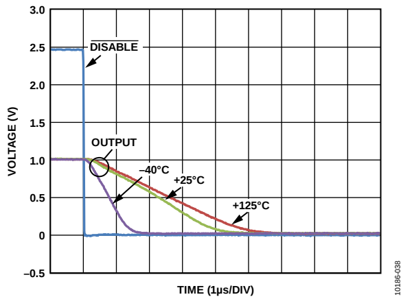
Figure 40. Output Turn-Off Time vs. Temperature
