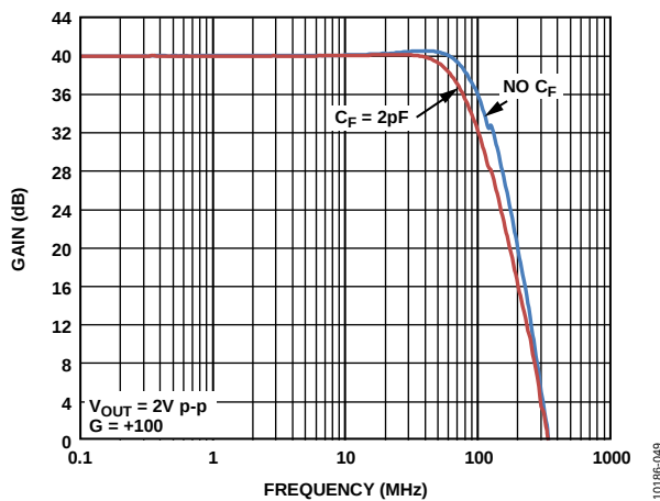
Figure 53. Large Signal Frequency Response, G = +100 , V_S = \pm 5 V
