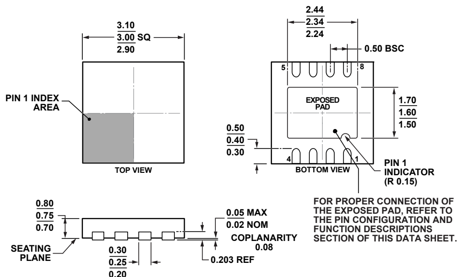
Figure 57. 8-Lead Lead Frame Chip Scale Package [LFCS_P_WD] 3 mm × 3 mm Body, Very Very Thin, Dual Lead (CP-8-11)
