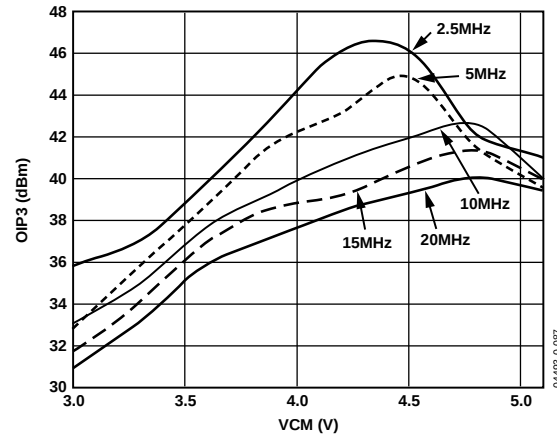
Figure 42. IOUTN Third-Order Intercept vs. Common-Mode Voltage (IAMP Settings of I = 12.5 \text{ mA} , N = 4 , G = 0 , 2:1 Transformer into 75 \Omega Load)
