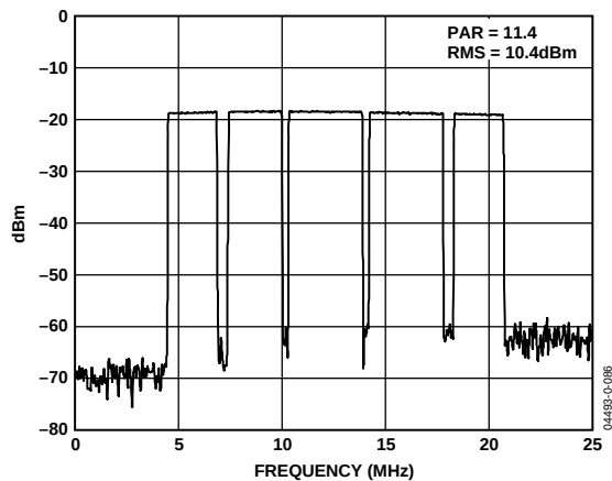
Figure 41. Spectral Plot of 84-Carrier OFDM Test Vector Using IAMP in Voltage-Mode Configuration with AV_{\text{DD}} = 5 \text{ V} (PBR951 Transistors, IAMP Settings of I = 6 \text{ mA} , N = 2 , G = 6 )
