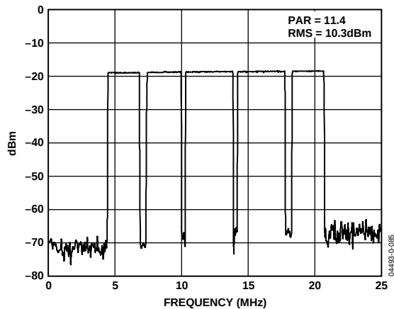
Figure 40. Spectral Plot of 84-Carrier OFDM Test Vector Using IAMPN in Current-Mode Configuration (IAMP Settings of I = 10 \text{ mA} , N = 4 , G = 0 ; V_{\text{CM}} = 4.8 \text{ V} )
