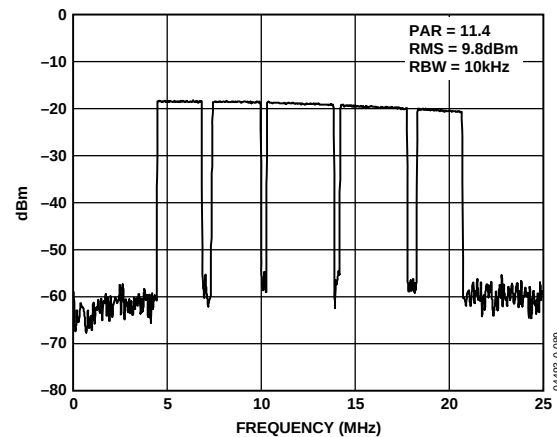
Figure 44. Spectral Plot of 84-Carrier OFDM Test Vector Using IAMP in Voltage-Mode Configuration with AV_{\text{DD}} = 3.3 \text{ V} (PBR951 Transistors, IAMP Settings of I = 6 \text{ mA} , N = 2 , G = 6 )
