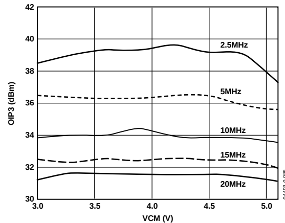
Figure 43. IOUTG Third-Order Intercept vs. Common-Mode Voltage (IAMP Settings of I = 4.25 \text{ mA} , N = 0 , G = 6 , 2:1 Transformer into 75 \Omega Load)
