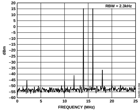
Figure 39. Dual-Tone Spectral Plot of IAMPN Output (IAMP Settings of I = 12.5 \text{ mA} , N = 4 , G = 0 , 2:1 Transformer into 75 \Omega Loader, V_{\text{CM}} = 4.8 \text{ V} )
