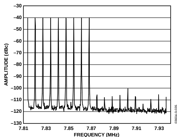
Figure 38. AD9863 Tx Path FFT, Upper-Band IMD Products of OFDM Signal in Figure 34
