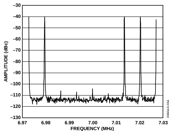
Figure 37. AD9863 Tx Path FFT, In-Band IMD Products of OFDM Signal in Figure 34
