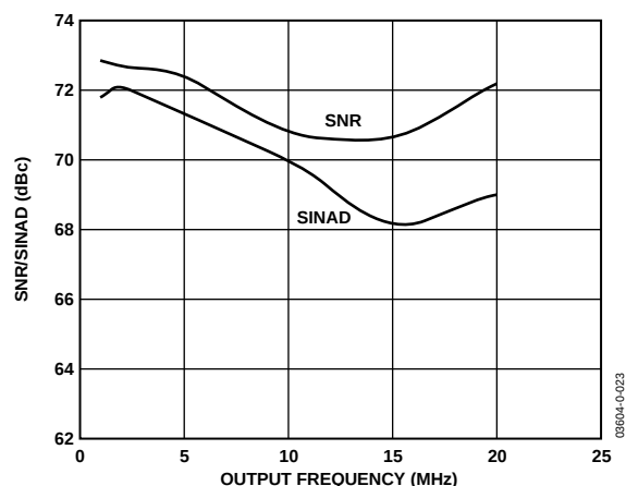
Figure 26. AD9863 Tx Path SINAD/SNR vs. Output Frequency of Tx Path with 20 mA Full-Scale Output into 60 \Omega Differential Load
