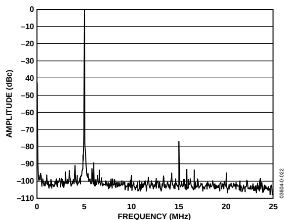
Figure 25. AD9863 Tx Path 5 MHz Single-Tone Output FFT of Tx Channel A with 20 mA Full-Scale Output into 33 \Omega Differential Load
