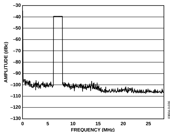
Figure 39. AD9863 Tx Path FFT of OFDM Signal in Figure 34, with 2 \times Interpolation
