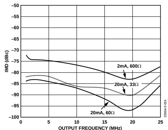
Figure 27. AD9863 Tx Path Dual-Tone (0.5 MHz Spacing) IMD vs. Output Frequency
