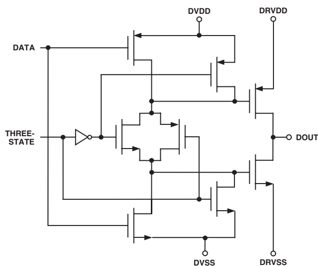
Figure 2. Data Outputs—D0–D13
