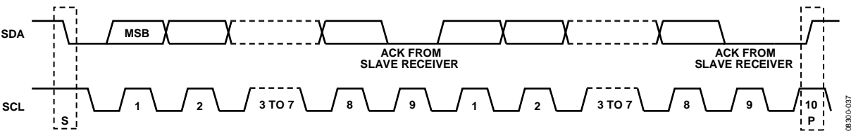
Figure 62. Acknowledge Bit
