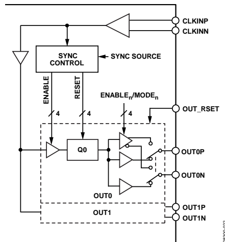
Figure 47. Clock Distribution
