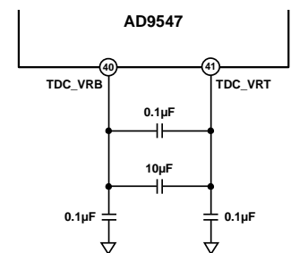
Figure 38. TDC Pin Connections
