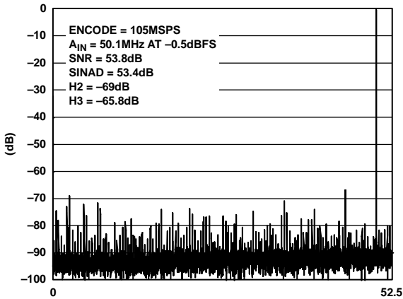
Figure 14. FFT: FS = 105 MSPS, A_{IN} = 50.1\text{ MHz @ } -0.5\text{ dBFS} , Differential, 1 V p-p Input Range
