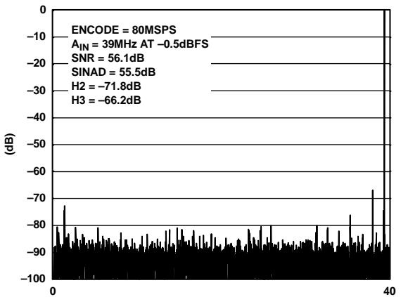
Figure 15. FFT: FS = 80 MSPS, A_{IN} = 39\text{ MHz @ } -0.5\text{ dBFS} , Differential, 1 V p-p Input Range
