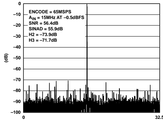
Figure 19. FFT: FS = 65 MSPS, A_{IN} = 15\text{ MHz @ } -0.5\text{ dBFS} ; with AD8138 Driving ADC Inputs, 1 V p-p Input Range
