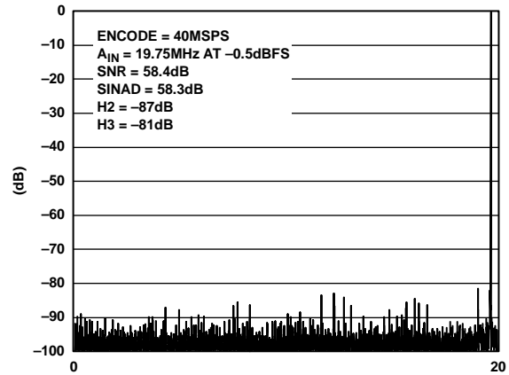
Figure 17. FFT: FS = 40 MSPS, A_{IN} = 19.75\text{ MHz @ } -0.5\text{ dBFS} , Differential, 1 V p-p Input Range
