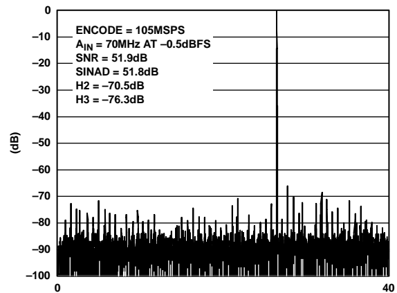
Figure 18. FFT: FS = 105 MSPS A_{IN} = 70\text{ MHz @ } -0.5\text{ dBFS} , Differential, 1 V p-p Input Range
