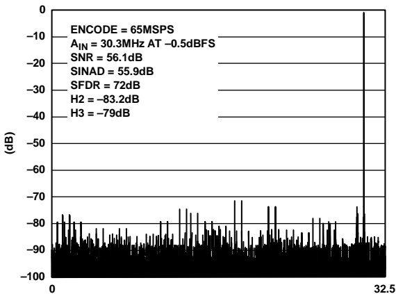
Figure 16. FFT: FS = 65 MSPS, A_{IN} = 30.3\text{ MHz @ } -0.5\text{ dBFS} , Differential, 2 V p-p Input Range
