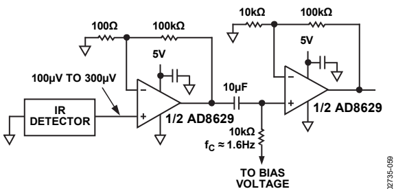
Figure 62. AD8629 Used as Preamplifier for Thermopile
