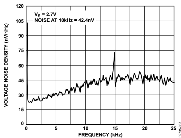
Figure 39. Voltage Noise Density at 2.7 V from 0 Hz to 25 kHz
