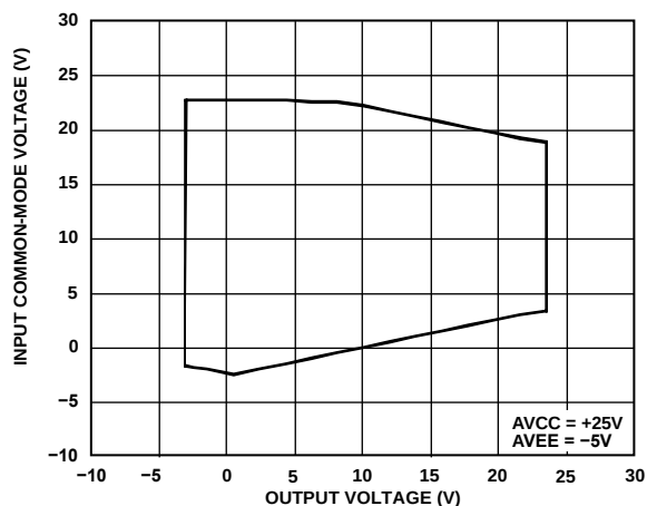
Figure 3. Input Common-Mode Voltage vs. Output Voltage for AV_{CC} = +25\text{ V} and AV_{EE} = -5\text{ V}
