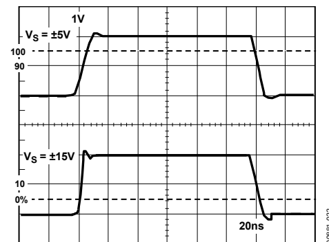
Figure 22. Large Signal Pulse Response, R_L = 150\Omega , C_L = 4.7pF , G = +1
