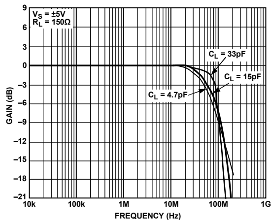
Figure 20. Closed-Loop Gain vs. Frequency vs. C_L , G = +1 , V_S = \pm 5V
