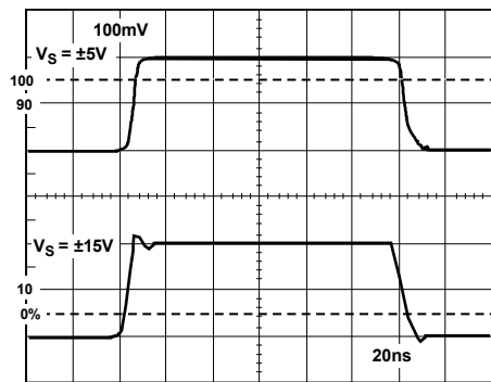
Figure 19. Small Signal Pulse Response, R_L = 150\Omega , C_L = 4.7pF , G = +1
