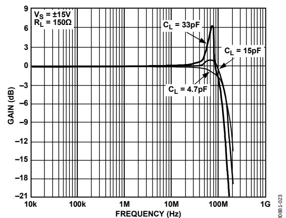
Figure 23. Closed-Loop Gain vs. Frequency vs. C_L , G = +1 , V_S = \pm 15V
