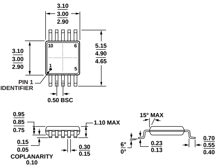
Figure 60. 10-Lead Mini Small Outline Package [MSOP] (RM-10)
