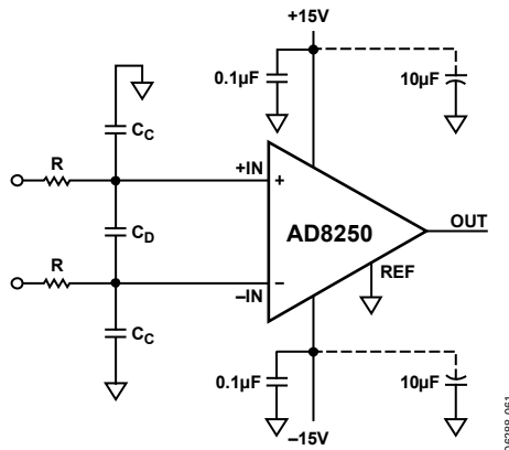
Figure 54. RFI Suppression
