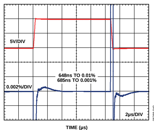
Figure 40. Large Signal Pulse Response and Settling Time G = 10, R_L = 10 \text{ k}\Omega
