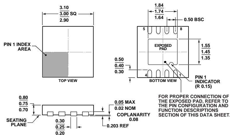
Figure 73. 8-Lead Lead Frame Chip Scale Package [LF CSP_WD]
