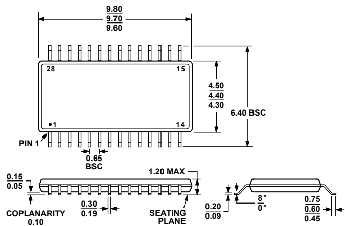
COMPLIANT TO JEDEC STANDARDS MO-153-AE Figure 30. 28-Lead Thin Shrink Small Outline Package [TSSOP] (RU-28) Dimensions shown in millimeters
