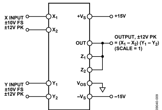
Figure 8. Connections for Scale Factor of Unity
