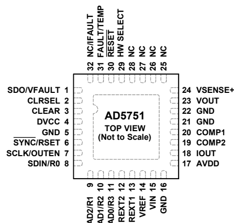
Figure 4. Pin Configuration
