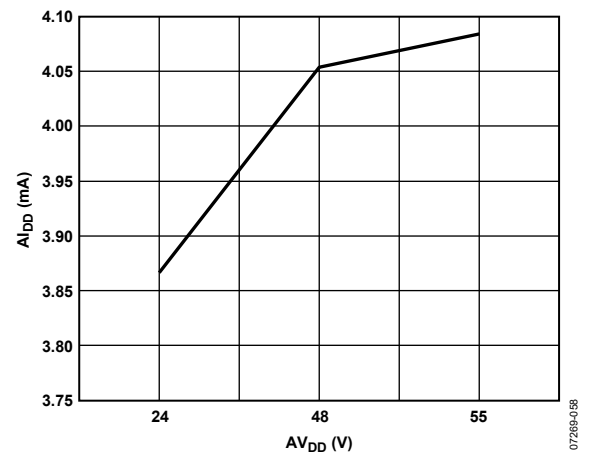
Figure 49. A_{IDD} vs. A_{VDD} , I_{OUT} = 0 mA
