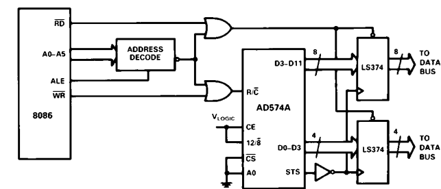
Figure 13. 8086 Stand-Alone Configuration
