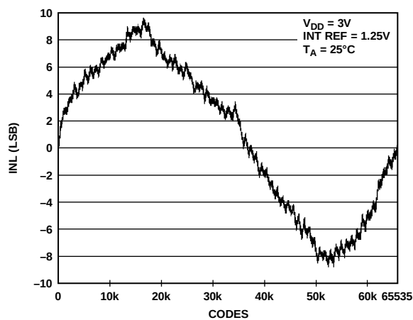
Figure 14. INL AD5669R-1—Internal Reference
