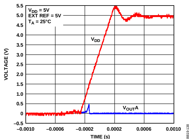
Figure 32. Power-On Reset to 0 V
