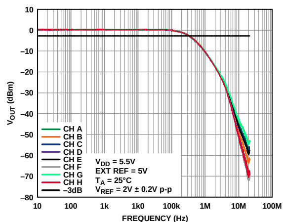
Figure 45. Multiplying Bandwidth
