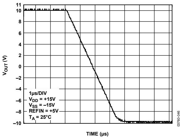
Figure 28. Settling Time
