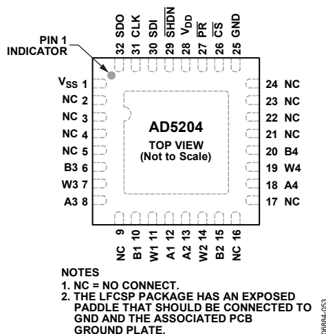
Figure 7. AD5204 LFCSP Pin Configuration
