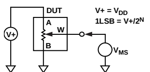
Figure 36. Potentiometer Divider Nonlinearity Error (INL, DNL)
