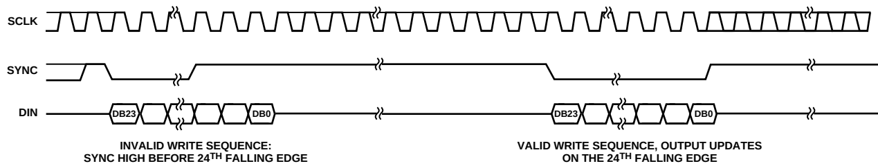
Figure 43. AD5060 \overline{\text{SYNC}} Interrupt Facility
