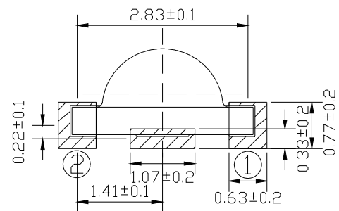
Recommend Soldering Pad
