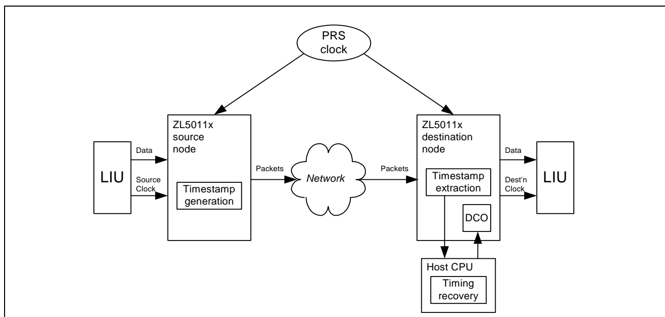
Figure 18 - Differential Clock Recovery
