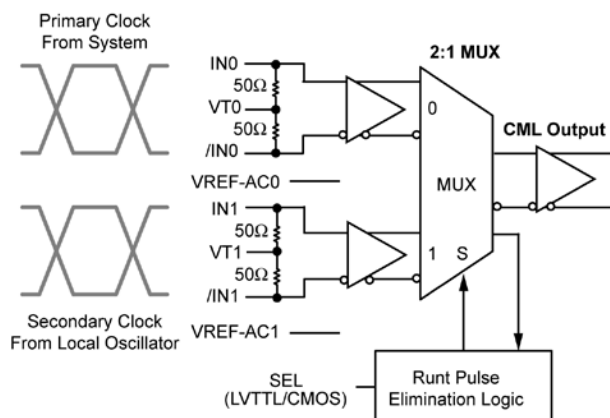
Simplified Example Illustrating Runt Pulse Eliminator (RPE) Circuit when Primary Clock Fails
