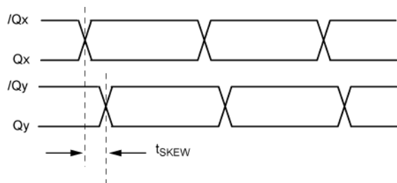
Output-to-Output Skew
