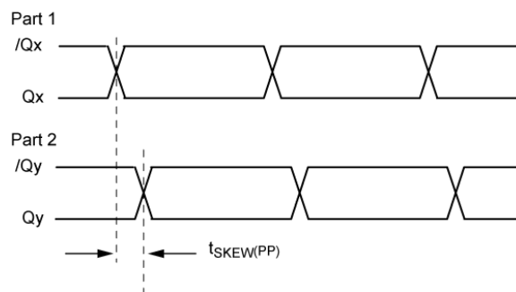
Part-to-Part Skew
